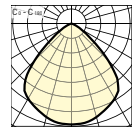
Ector M73 RSM 314...TWLi 830
