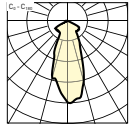
Combial SM/1x70 HIT-DE...TW nw
