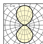
Luceo H CDP LED 4000-840... UTE: 0,48 D + 0,52 T DIN 5040: C43 CIBSE: BZ 2/1.75/BZ 3 NBN L 14-002: BZ 3
